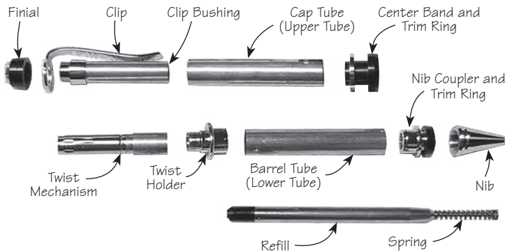
Pen parts.
